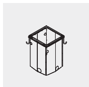
CA275/600 Foundation box for SPARTACUS 275 h 600 mm.
